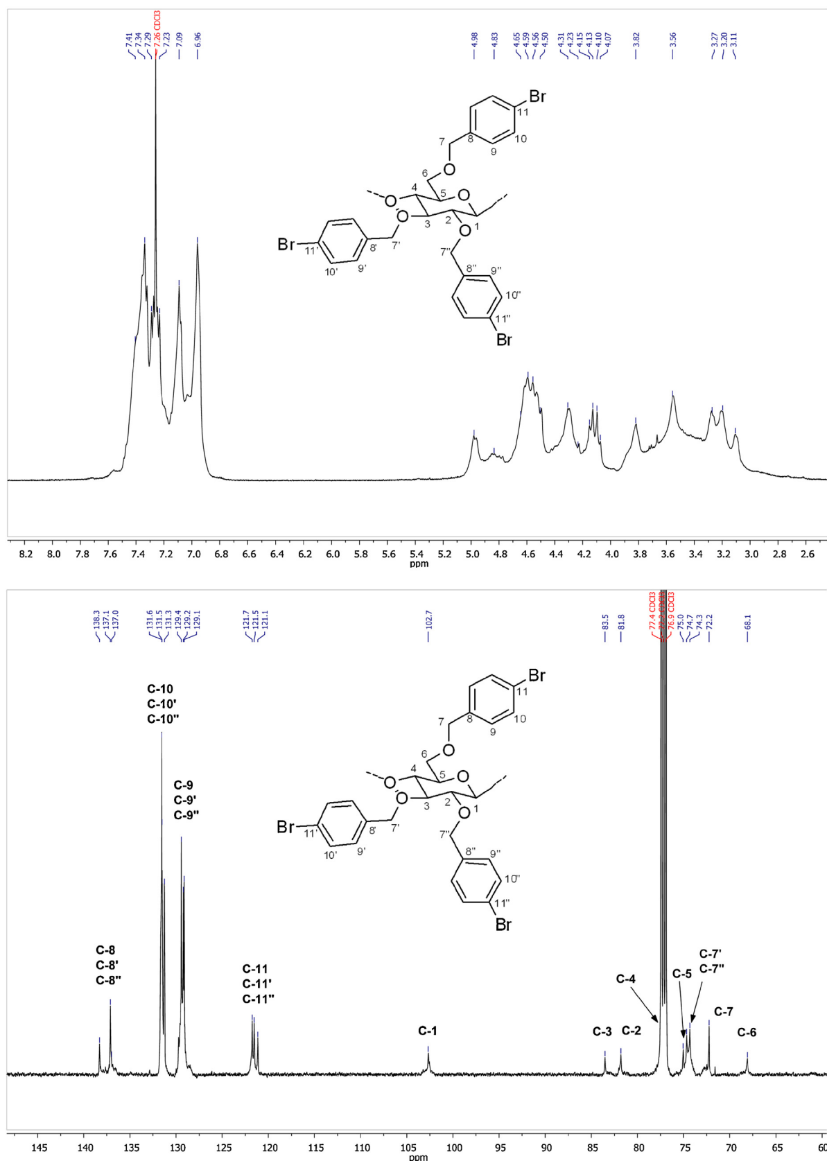
Fig. 3. ^1\text{H} - and ^{13}\text{C} NMR spectra of cellulose ether 2c in \text{CDCl}_3 .
